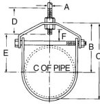
C-710 Adjustable Clevis Hanger
