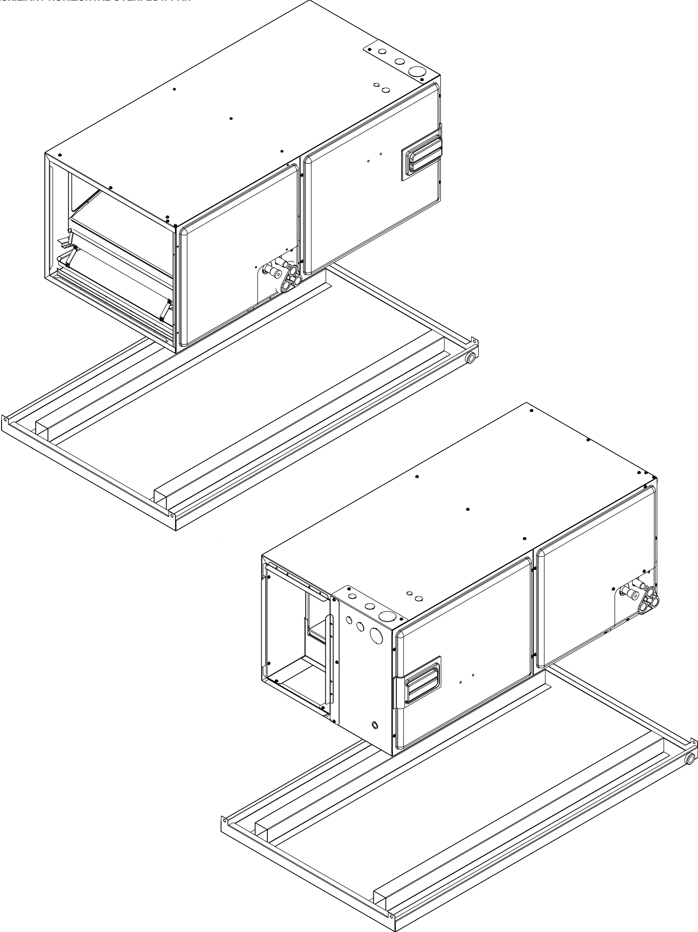
FIGURE 1 AUXILIARY HORIZONTAL OVERFLOW PAN
