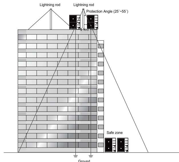
Figure 49: Lightning Protection Diagram.
