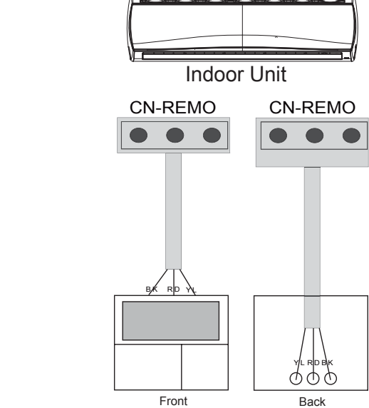
Figure 46: Another Example of Indoor Unit to Zone Controller Connection.
