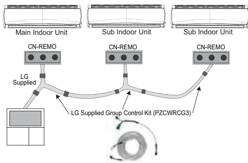
Figure 48: Example of Indoor Unit Group to Zone Controller Connections (CN-REMO).
