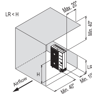
Figure 59: Proper Outdoor Unit Placement and Clearances.
