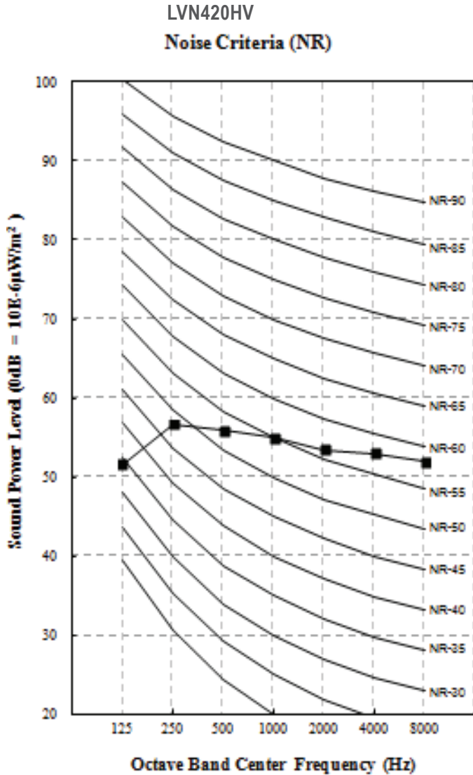
Figure 17: LVN420HV Sound Power Level Diagram.
