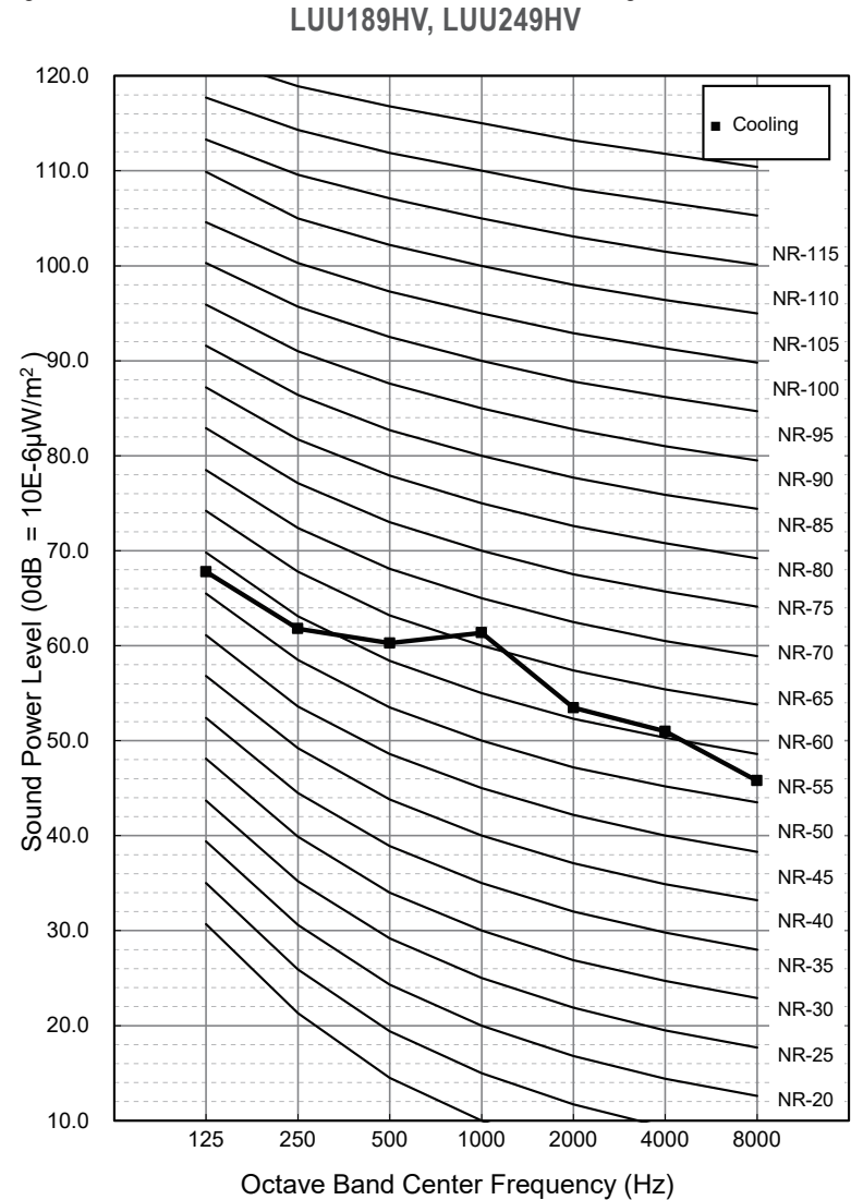
Figure 23: LUU189HV, LUU249HV Sound Power Level Diagram.
