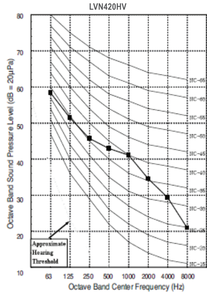
Figure 12: LVN420HV Sound Pressure Level Diagram.
