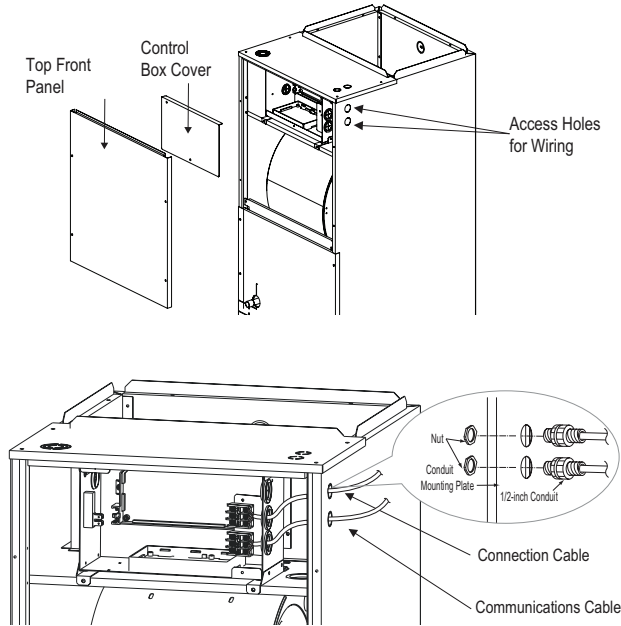
Figure 37: Connecting the Power Wiring and Communications Cable.
