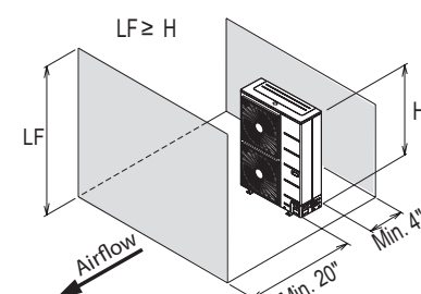
Figure 60: Proper Outdoor Unit Placement and Clearances, continued.
