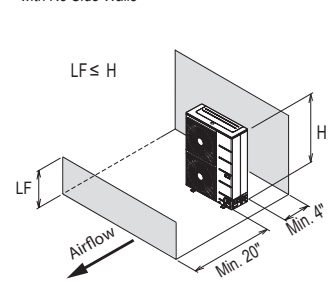
Figure 59: Proper Outdoor Unit Placement and Clearances.
